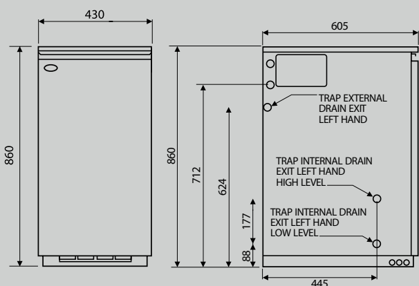
Grant Vortex Eco 15-21 and 21-26 Utility and System
