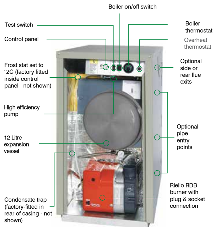
Model shown: VTXSOMECO15/21 (front view)
