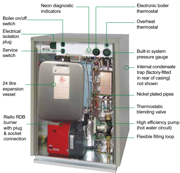
Model shown: VTXOMCOMBI26 (front view)
