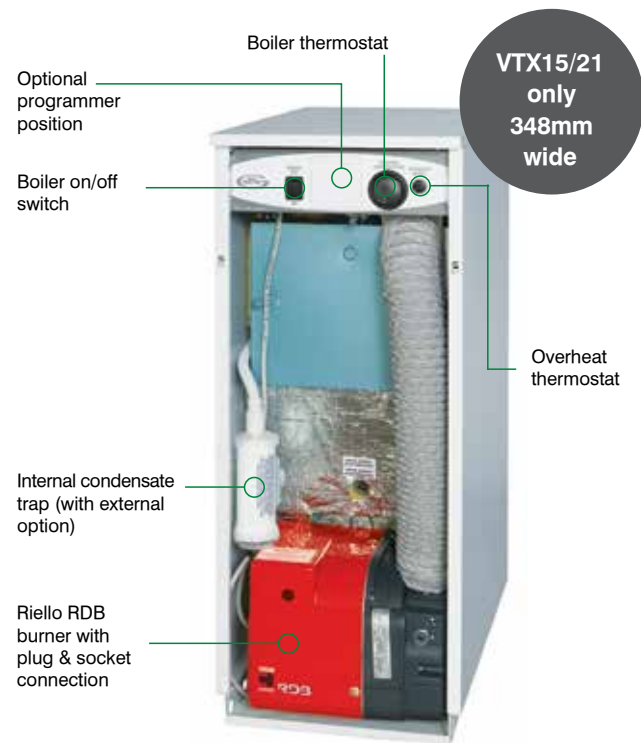
Model shown: VTX15/21 (front view)
