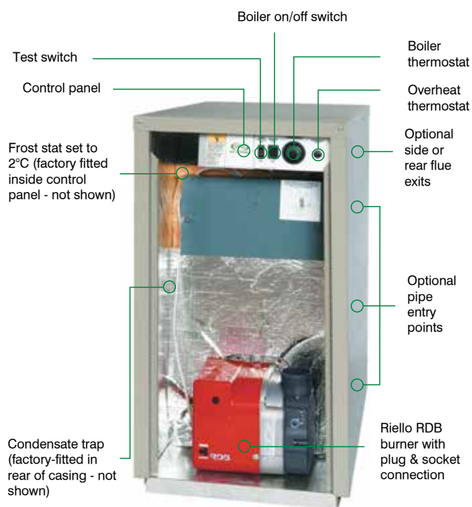
Model shown: VTXOMECO15/21 (front view)
